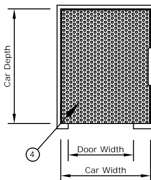
Floor Plan
