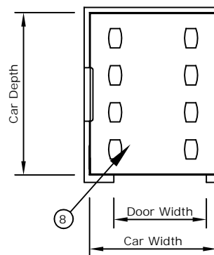
Ceiling Plan
