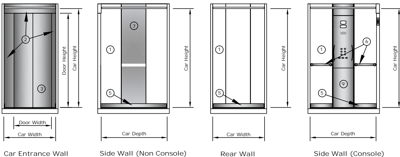
Typical open front laminate car arrangement (8 person / 630 Kg capacity white carrara laminate car shown)
